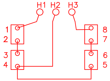
HEATER HOOKUP
