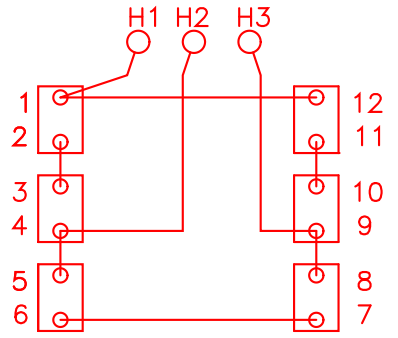
HEATER HOOKUP
